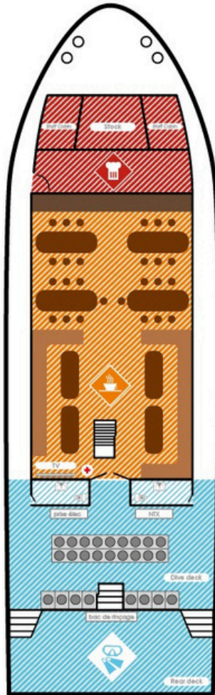
MAIN DECK
